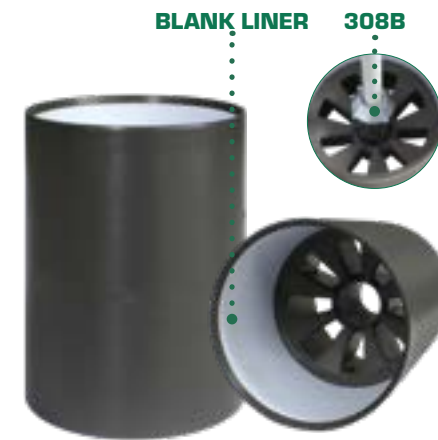
Aluminum Pro Hole Cup [No. 253AL-3] This cup is made of durable heat treated aluminum alloy. Accepts British/locking [308B] ferrule to complete locking mechanism (pg. 28/29).
