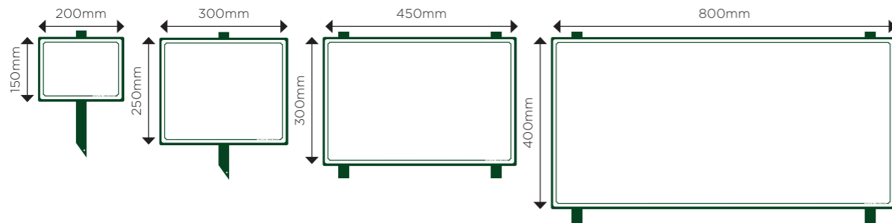
SPIKE 5114, PLATE 5115
